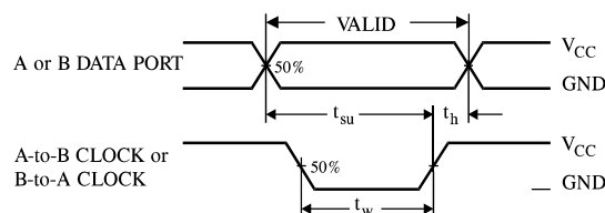
Figure 7. Switching Waveforms
