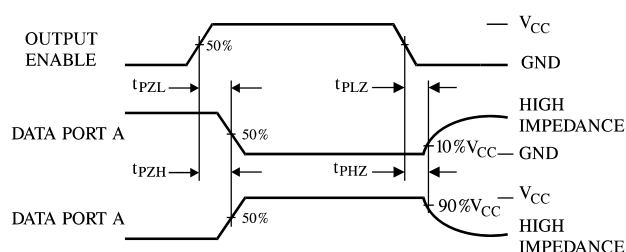
Figure 5. Switching Waveforms
