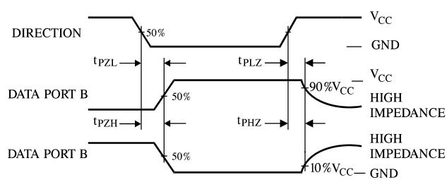
Figure 6. Switching Waveforms
