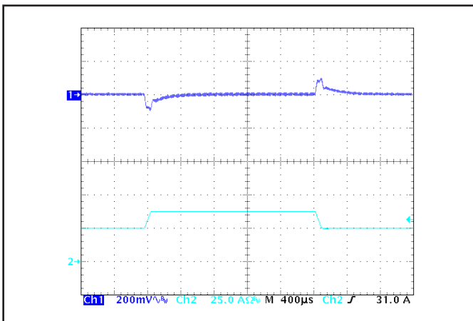
Figure 5: Output voltage response to step-change in load current (50%-75%-50% of I out (max); dl/dt = 0.2 A/µs). Load cap: 1 µF ceramic and 15 µF tantalum capacitors. Ch 1: V out (200 mV/div), Ch 2: I out (25 A/div).
