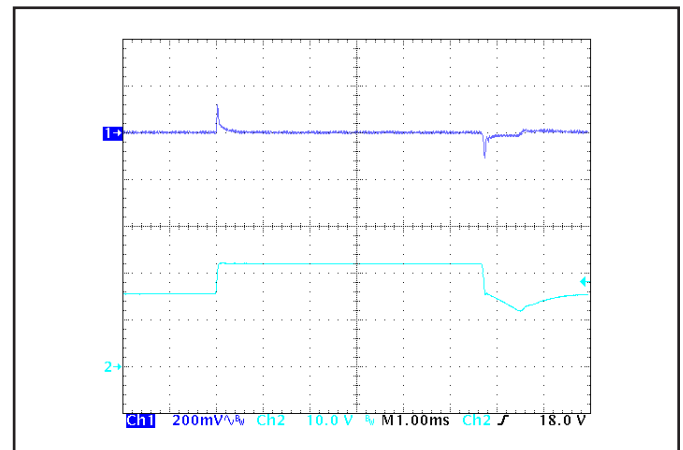
Figure 6: Output voltage response to step-change in input voltage (500 V/ms). Load cap: 100 µF, electrolytic output capacitance. Ch 1: V out (200 mV/div), Ch 2: V in (10 V/div).
