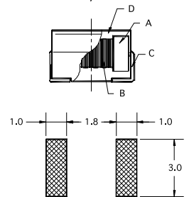
Pad layout
