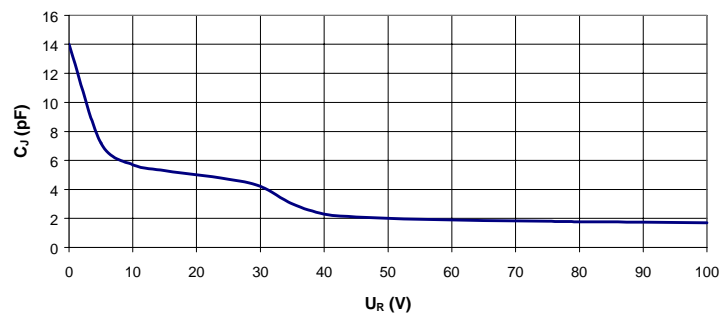
C_J (pF)= U_R (AD230)
