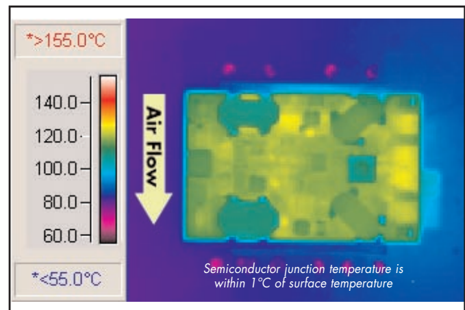
Figure 12: Thermal plot of converter at 12A load on 1.5V output and 9.5A load on 3.3V output with 85°C air flowing at 200 LFM. Air flow across the converter is from pin 1 to pin 3 (nominal input voltage).
