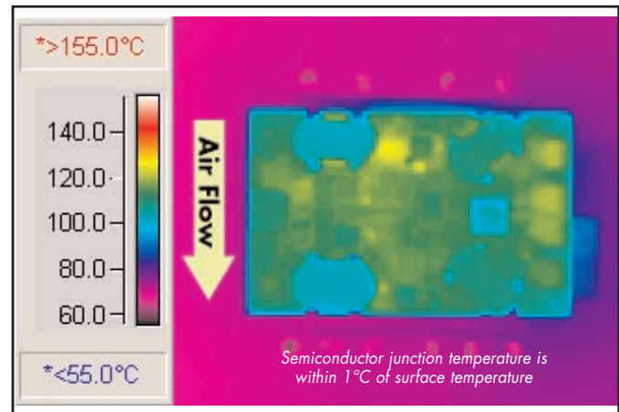
Figure 10: Thermal plot of converter at 13A load on 1.5V output and 12.5A load on 3.3V output with 70°C air flowing at 200 LFM. Air flow across the converter is from pin 1 to pin 3 (nominal input voltage).
