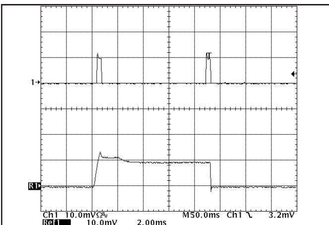
Figure 23: Load current for 1.5V output (20A/div) as a function of time when the converter attempts to turn on into a 10 m\Omega short circuit. Bottom trace is an expansion of the on-time portion of the top trace.
