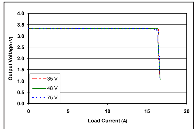
Figure 22: Output voltage vs. load current showing typical current limit curves and converter shutdown points for the 3.3V output. 1.5V load is at 0A.
