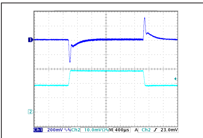
Figure 5: Output voltage response to step-change in load current (50%-75%-50% of I out (max)); dI/dt = 0.1 A/µs. Load cap: 1 µF ceramic and 15 µF tantalum capacitors. Ch 1: V out (200 mV/div), Ch 2: I out (5 A/div).
