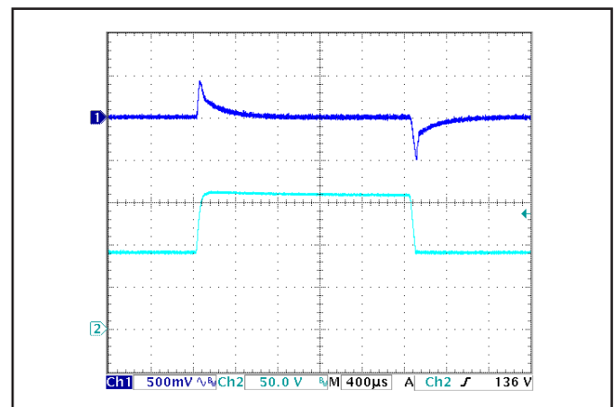
Figure 6: Output voltage response to step-change in input voltage (1000 V/ms). Load cap: 100 µF, electrolytic output capacitance. Ch 1: V out (500 mV/div), Ch 2: V in (50 V/div).
