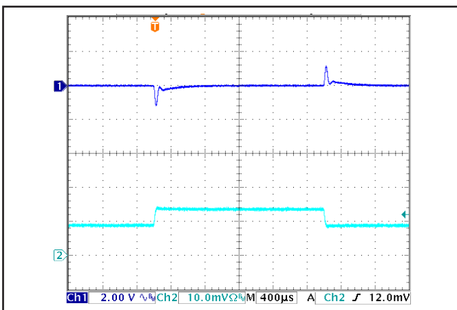
Figure 5: Output voltage response to step-change in load current (50%-75%-50% of Iout(max)); dl/dt = 0.1 A/us). Load cap: 1 μF ceramic capacitor. Ch 1: Vout (2 V/div), Ch 2: Iout (5 A/div).
