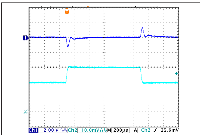
Figure 5: Output voltage response to step-change in load current (50%-75%-50% of Iout(max)); di/dt = 0.1 \text{ A}/\mu\text{s} . Load cap: 1 \mu\text{F} ceramic capacitor. Ch 1: Vout (2 V/div), Ch 2: Iout (2 A/div).
