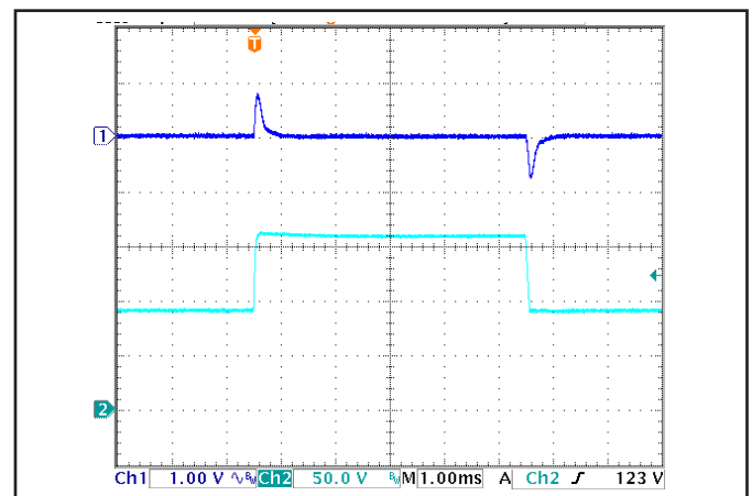
Figure 6: Output voltage response to step-change in input voltage (1000 V/ms). Load cap: 100 \mu\text{F} , electrolytic output capacitance. Ch 1: Vout (1 V/div), Ch 2: Vin (50 V/div).
