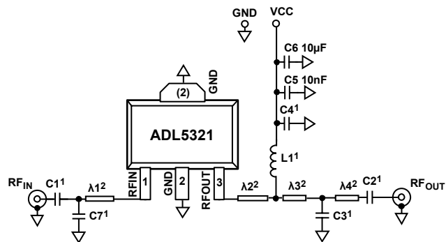
Figure 20. Basic Connections
