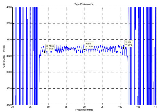
Group Delay Variation(f0±11MHz)
