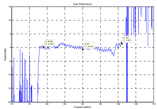
Phase Linearity(f0±11MHz)
