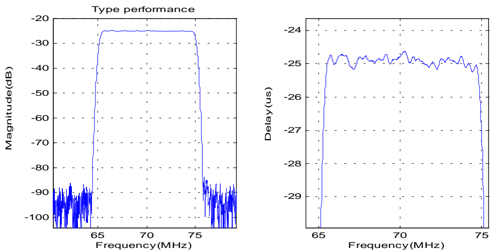
LBN7020N SAW Filter Typical Performance
