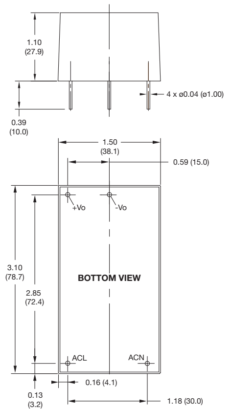
Encapsulated (-E)
