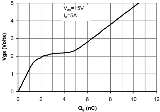
Figure 7: Gate-Charge Characteristics
