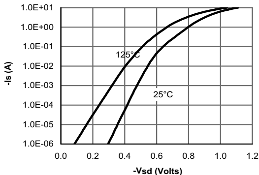
Figure 6: Body-Diode Characteristics
