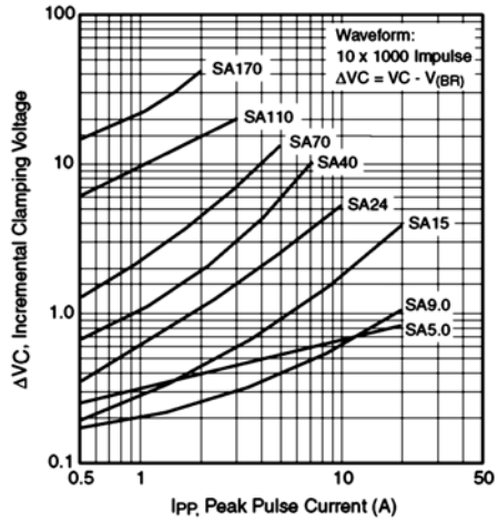
Fig. 8 – Incremental Clamping Voltage Curve Unidirectional
