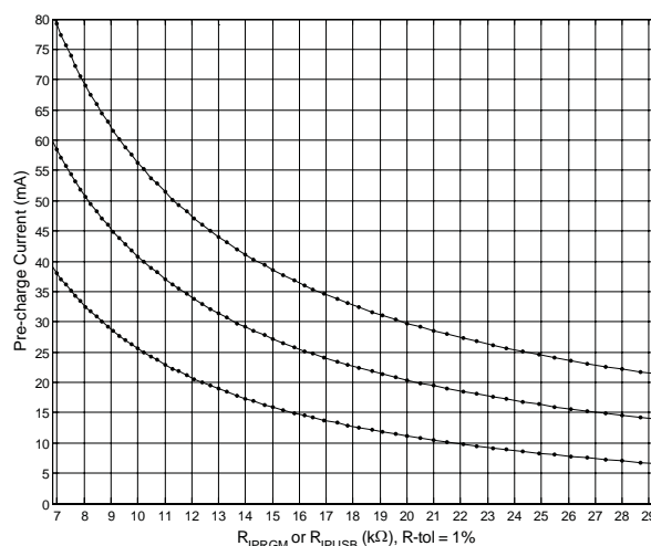
Figure 2b — Pre-charge Current Tolerance versus Programming Resistance, High Resistance Range
