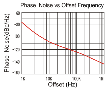
SMO-8D
