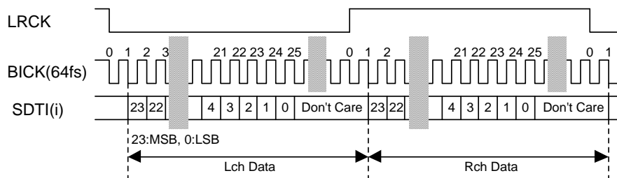
Figure 4. Mode 2 Timing
