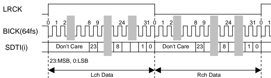
Figure 5. Mode 3 Timing
