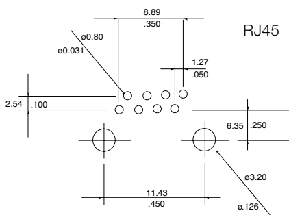
PC Board Layout 8x8
