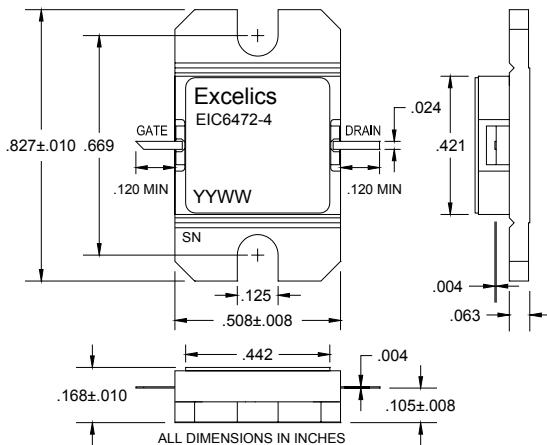
EIC6472-4 (Hermetic)
