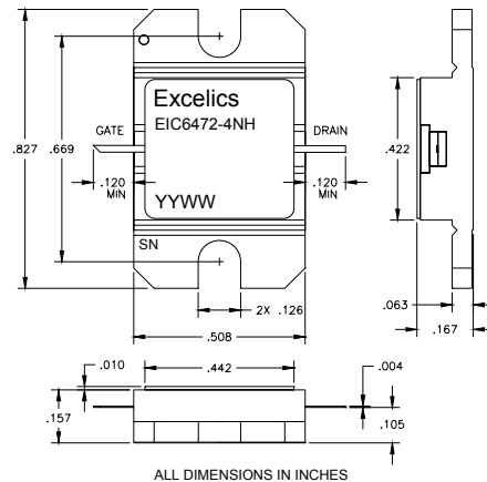
EIC6472-4NH (Non-Hermetic)
