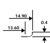
Detail of Contacts B
