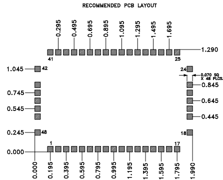
PACKAGE MOUNTING: SEE APPLICATION NOTE AN7200 TOLERANCES ON THREE DECIMAL PLACES = ± 0.015
