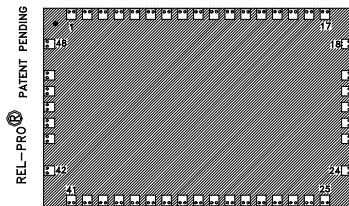
PACKAGE MOUNTING: SEE APPLICATION NOTE AN7200 TOLERANCES ON THREE DECIMAL PLACES = ± 0.015
