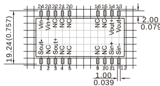
Pin Connection
