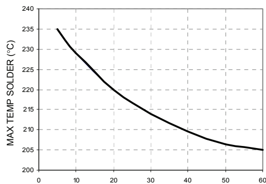
Figure 29. Time Limit Curve Above 205°C for Tin/Lead (Sn/Pb) process
