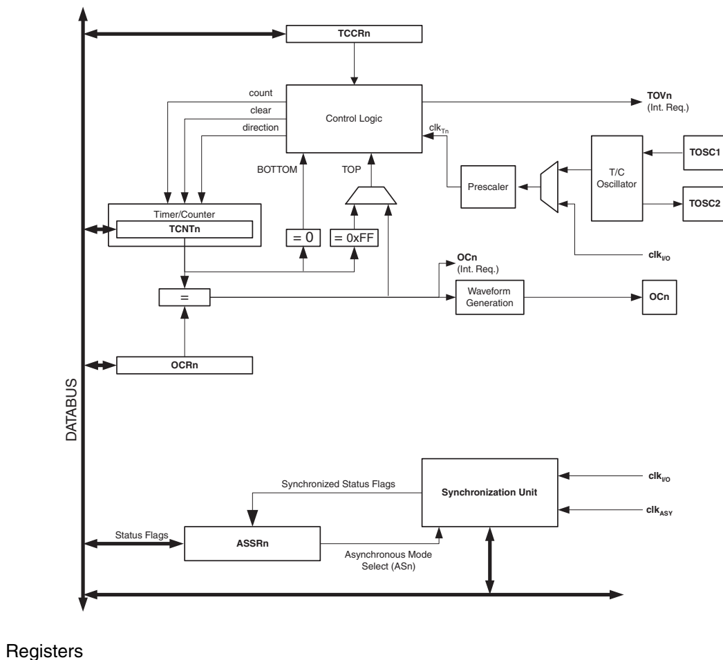
Figure 14-1. 8-bit Timer/Counter Block Diagram.
