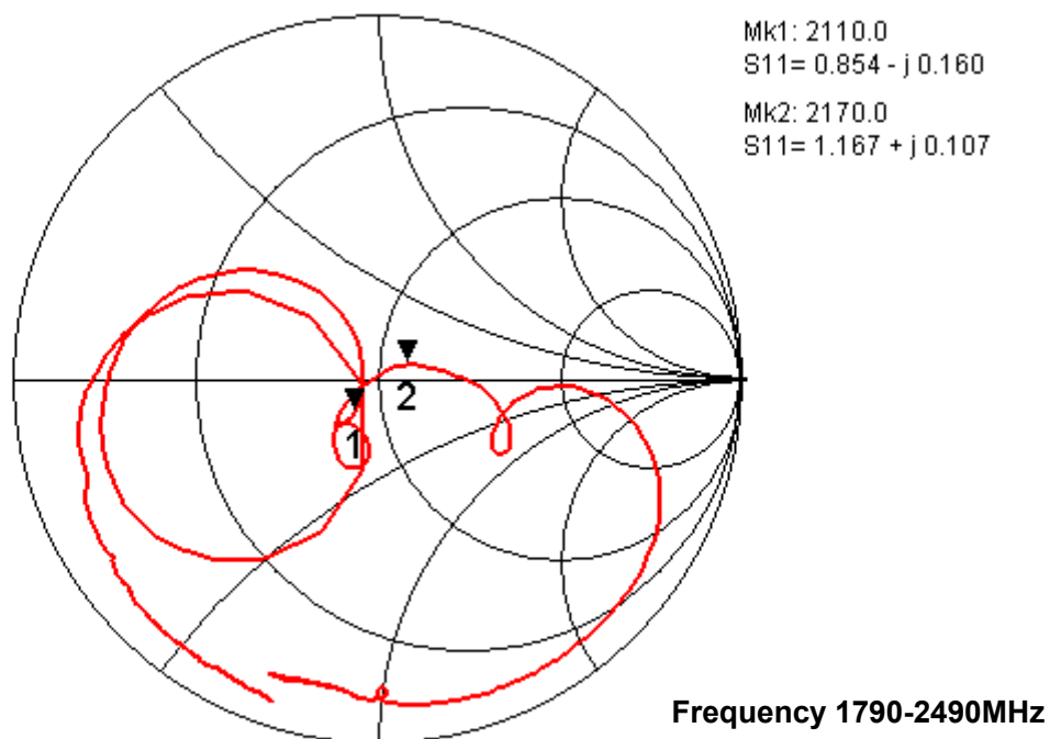
Fig.6 Impedance (unbal)
