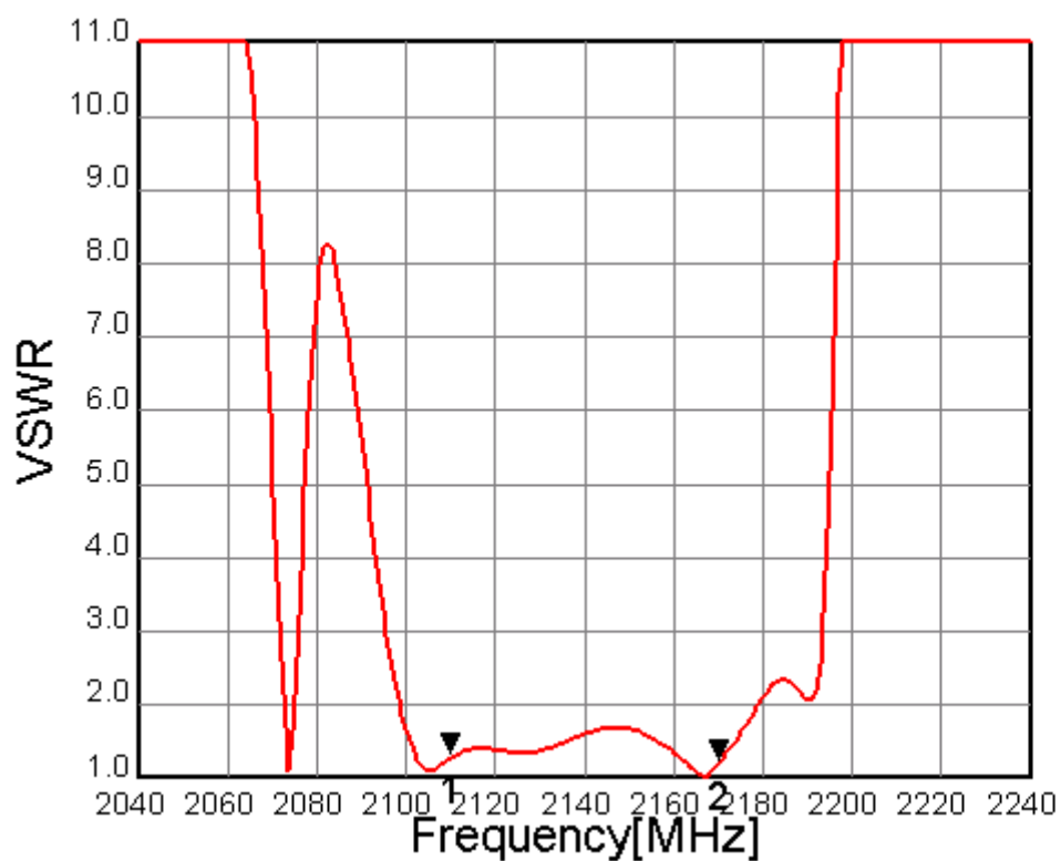
Fig.3 VSWR (unbal)
