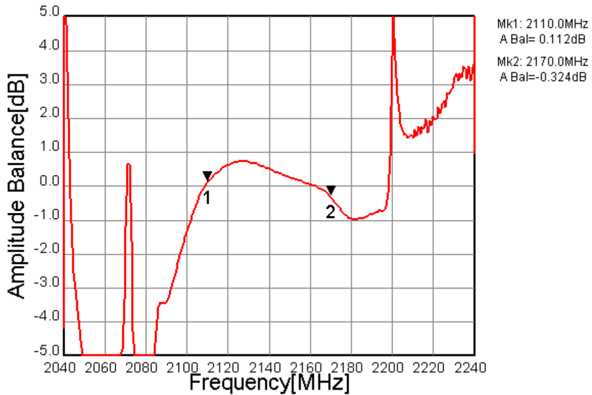
Fig.8 Amplitude Balance
