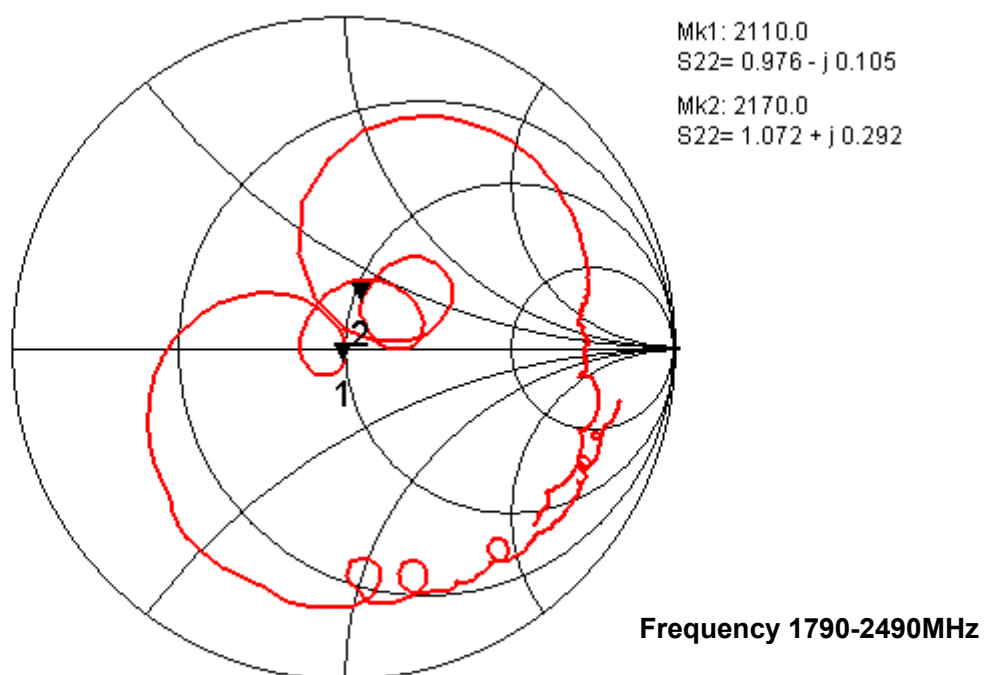
Fig.6 Impedance (unbal)
