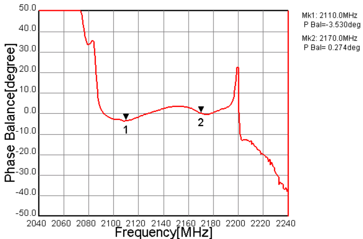
Fig.9 Phase Balance
