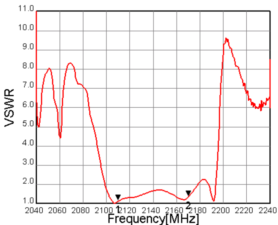
Fig.4 VSWR(bal)
