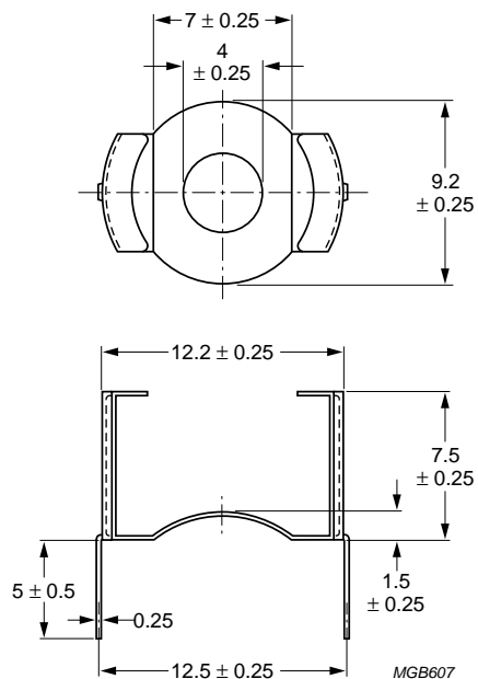
Fig.7 Clamp: CLM/TP-P11/7.
