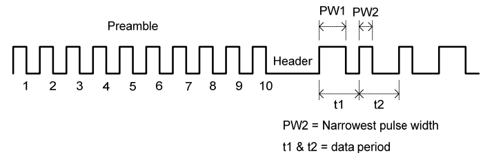
Figure 8. Example of a Data Profile.
