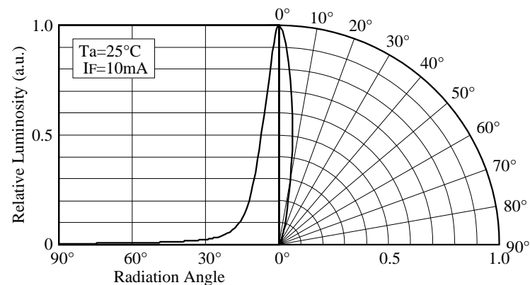
■ Directivity (NEPW500)
