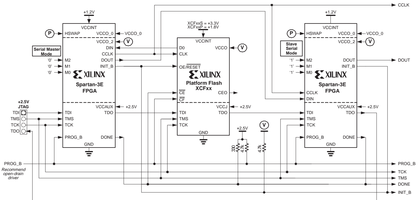
Figure 49: Daisy-Chaining from Master Serial Mode
