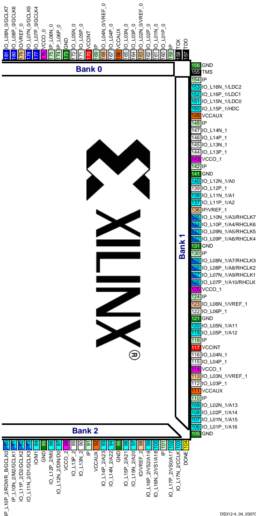
Figure 6: PQ208 Footprint (Right)
