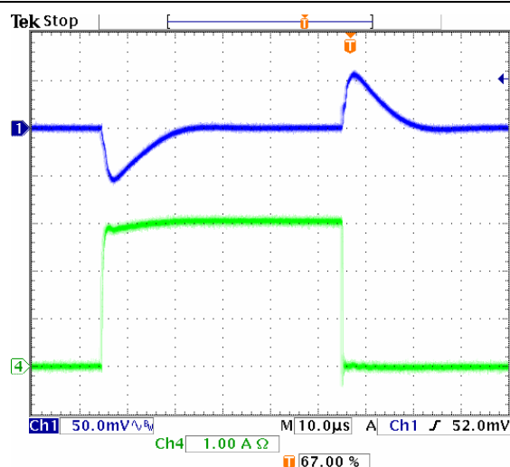
Load Transient: V_{IN} = 3.3V , V_{OUT} = 1.2V Ch.1: V_{OUT} , Ch.4: I_{LOAD} (slew rate \geq 10A/\mu s ) C_{IN} = 22\mu F , C_{OUT} \approx 50\mu F
