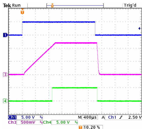
Power Up/Down into 0.4\Omega load: V_{IN}/V_{OUT} = 5.0V/1.2V , 15nF soft-start capacitor, Ch.1: ENABLE, Ch.3: V_{OUT} , Ch.4: POK
