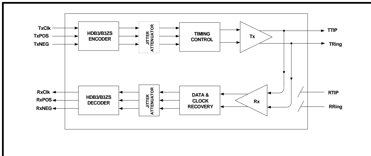
FIGURE 18. ANALOG LOOPBACK
