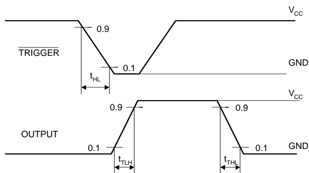
Figure 1. Switching Waveforms
