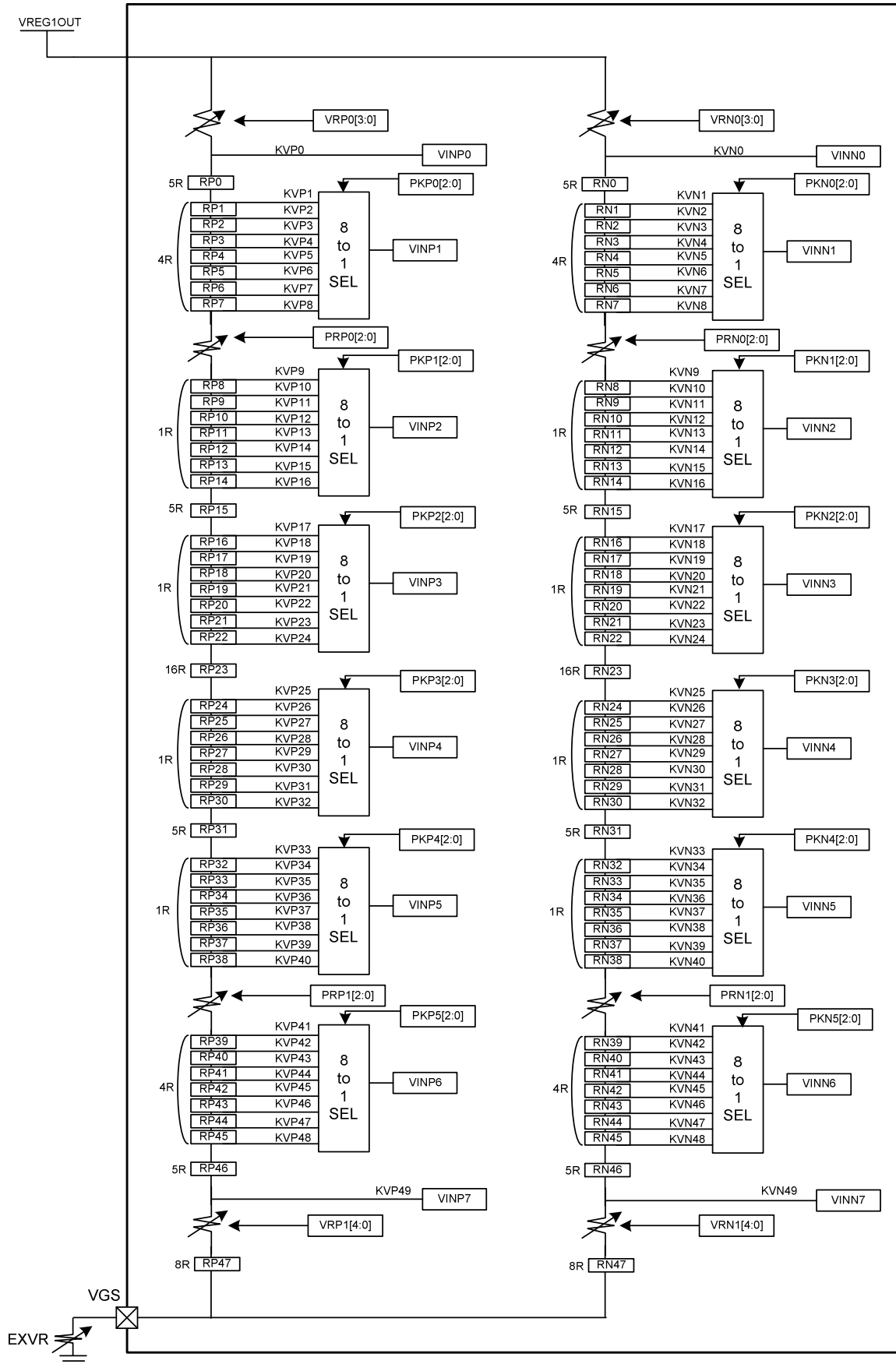
Structure of Ladder / 8 to 1 selector
