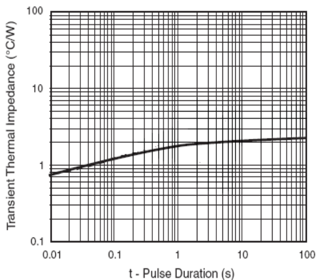
Figure 6. Typical Transient Thermal Impedance Per Diode
