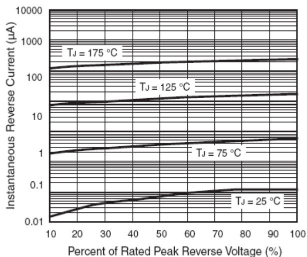
Figure 4. Typical Reverse Characteristics Per Diode
