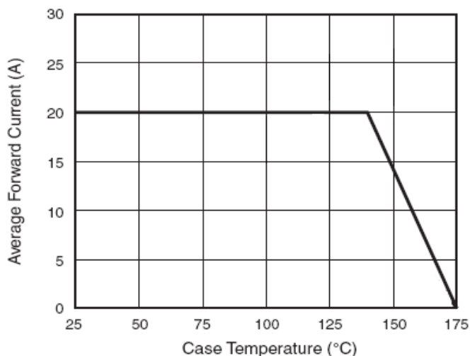
Figure 1. Forward Derating Curve (Total)
