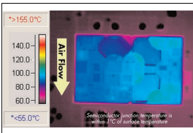
Figure 12: Thermal plot of converter at 15 amp load on 2.5V output and no load on 3.3V output with 55°C air flowing at 200 LFM. Air flow across the converter is from pin 1 to pin 3 (nominal input voltage)
