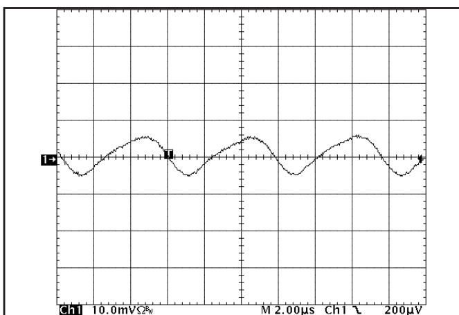
Figure 24: Input Terminal Ripple Current, 2.5V & 3.3V outputs at 50% rated output current and nominal input voltage with 10μH source impedance and 100μF electrolytic capacitor (200 mA/div). (see Fig. 23)
