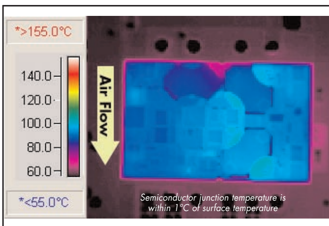
Figure 18: Thermal plot of converter at 4.8 amp load on 2.5V output and 8.5 amp load on 3.3V output with 55°C air flowing at 200 LFM. Air flow across the converter is from pin 1 to pin 3 (nominal input voltage).
