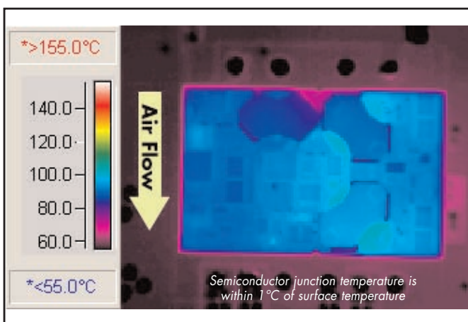
Figure 16: Thermal plot of converter at 8 amp load on 2.5V output and 6 amp load on 3.3V output with 55°C air flowing at 200 LFM. Air flow across the converter is from pin 1 to pin 3 (nominal input voltage)
