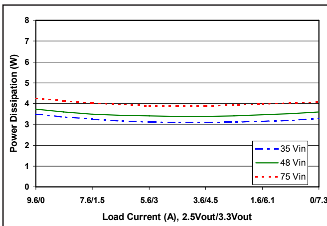
Figure 4: Power dissipation vs. load current, with total output power fixed at 60% load (24W) and load currents split as shown between 2.5V and 3.3V outputs at minimum, nominal, and max input voltage at 25°C.
