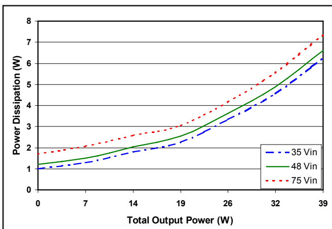
Figure 2: Power dissipation vs. output power, from 0 load to full load with 50% load on 2.5V output and 50% load on 3.3V output at minimum, nominal, and maximum input voltage at 25°C.
