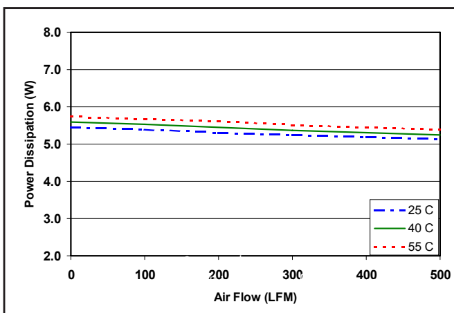
Figure 6: Power dissipation at 80% load and 50/50 voltage split (6.4A load on 2.5V and 4.8A load on 3.3V) versus airflow rate for ambient air temperatures of 25°C, 40°C, and 55°C (nominal input voltage).
