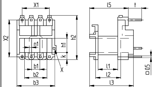
Sketch with main dimensions
