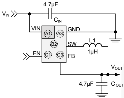
Figure 1. WLCSP (top view)
