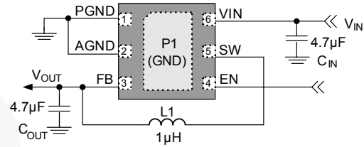
Figure 2. MLP (top view)
