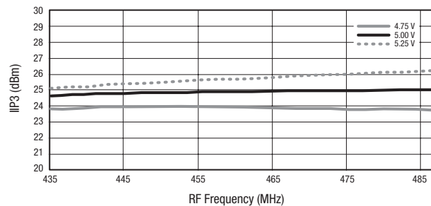
Figure 14. Mixer B IIP3 vs Frequency and Supply Voltage
