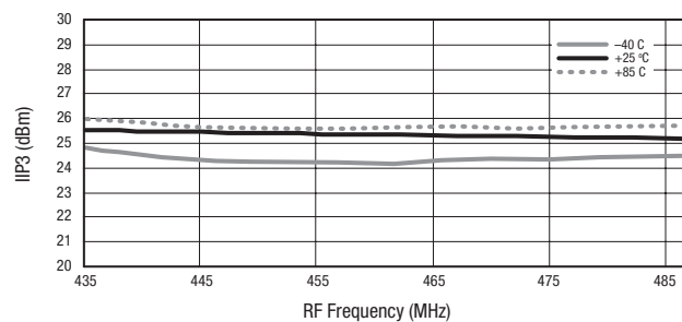
Figure 12. Mixer A IIP3 vs Frequency and Temperature
