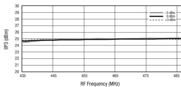
Figure 16. Mixer B IIP3 vs Frequency and LO Power
