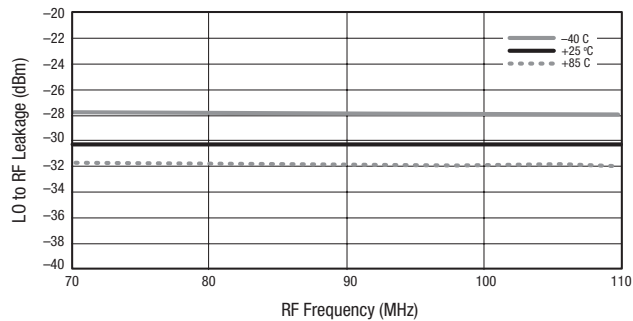
Figure 23. Mixer A LO to RF Leakage vs Frequency and Temperature
