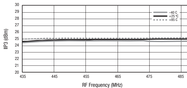
Figure 15. Mixer B IIP3 vs Frequency and Temperature
