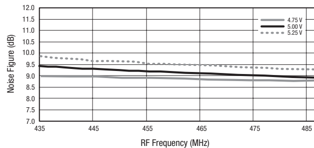
Figure 10. Mixer B Noise Figure vs Frequency and Supply Voltage
