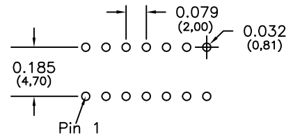
Recommended P.C. Board Layout 08 Style
