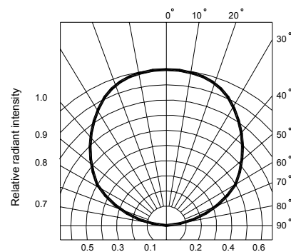
Fig.6 Radiation diagram
