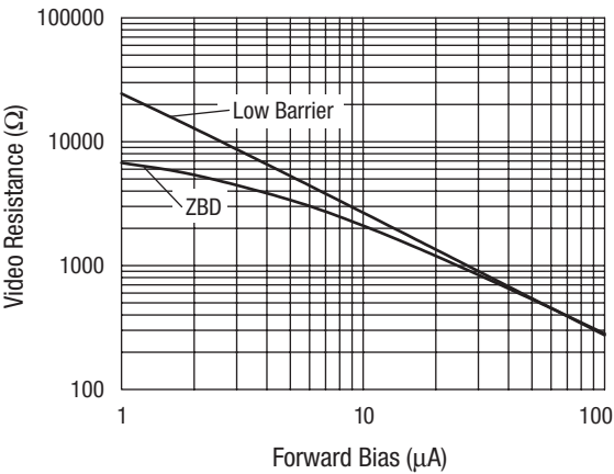
Figure 2. Video Resistance vs. Forward Bias Current
