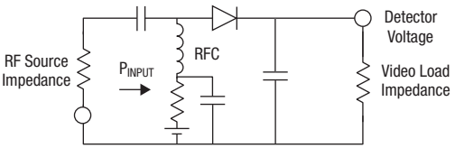
Biased Detector
