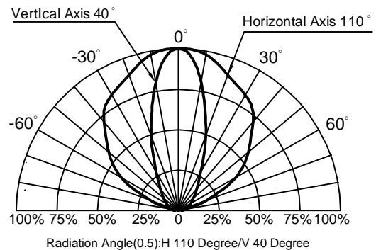
Fig.6 Directivity Radiation
