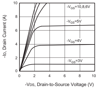
Figure 1. Output Characteristics
