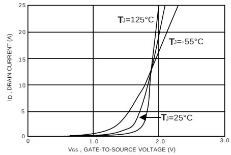
Figure 2. Transfer Characteristics
