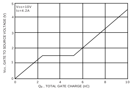
Figure 3. Gate Charge
