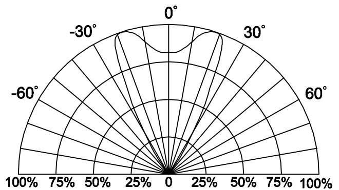
Fig.6 Directivity Radiation
