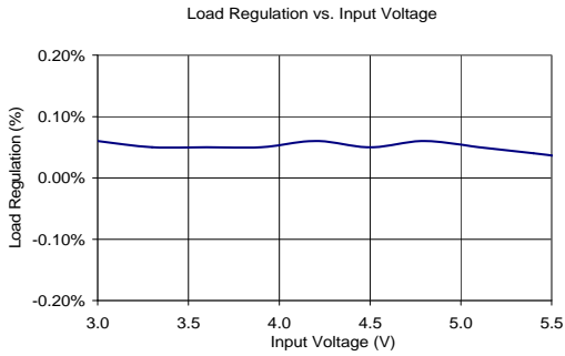
Figure 42: Load Regulation vs. Input Voltage
