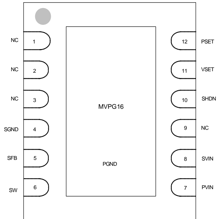
Figure 3: 12-Pin DFN Pin Diagram—MVPG16 Top View
