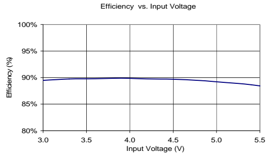
Figure 41: Efficiency vs. Input Voltage
