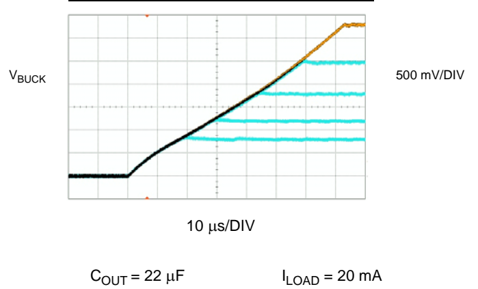
Figure 7: Soft Startup (0.8V, 1.2V, 1.8V, 2.5V, 3.3V)
