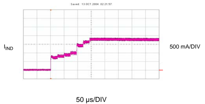
Figure 21: Soft Start Current Limit Steps
