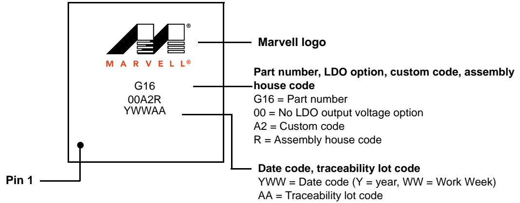
Figure 72: MVPG16 Package Marking
