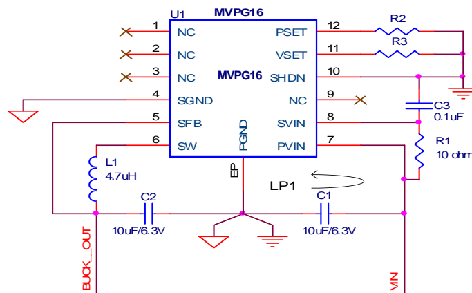
Figure 61: MVPG16 PCB Layout Schematic
