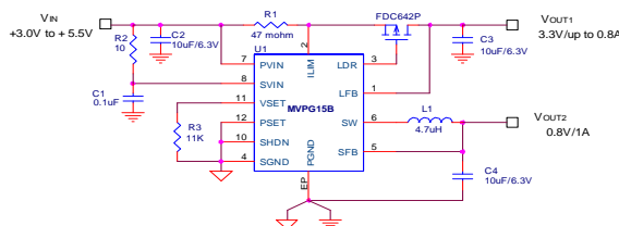
Figure 1: Typical High Efficiency 5.0V to 0.8V/3.0A Step-Down Regulator with 3.3V LDO Regulator
