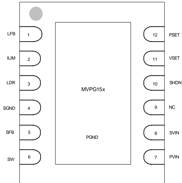
Figure 2: 12-Pin DFN Pin Diagram—MVPG15x Top View
