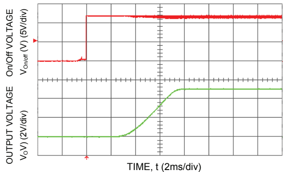
Figure 15. Typical Start-Up Using Remote On/Off with Low-ESR external capacitors ( 7 \times 150 \mu\text{F} Polymer) ( V_{in} = 12\text{Vdc} , V_o = 5.0\text{Vdc} , I_o = 16\text{A} , C_o = 1050 \mu\text{F} ).
