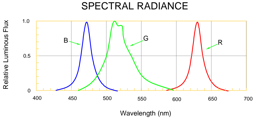
Fig.5 Luminous Spectrum( T_a=25 )
