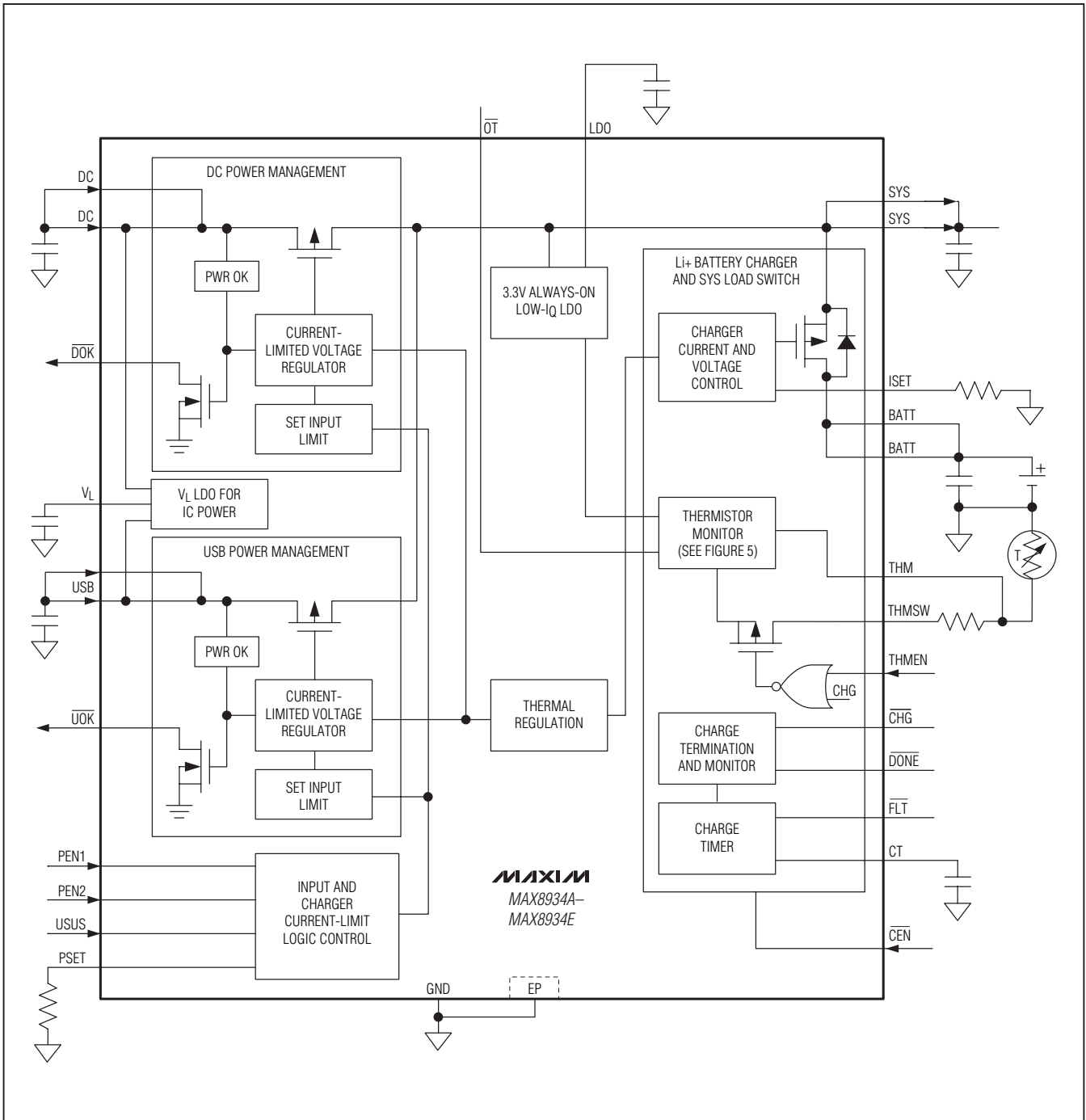
Figure 1. Block Diagram
