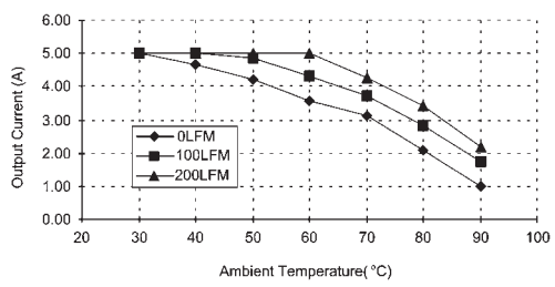
Standard Version Derating Curve for 3.3 VDC Output
