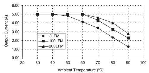
SMT Version Derating Curve for 3.3 VDC Output
