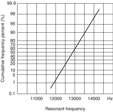
(4) Resonant frequency
